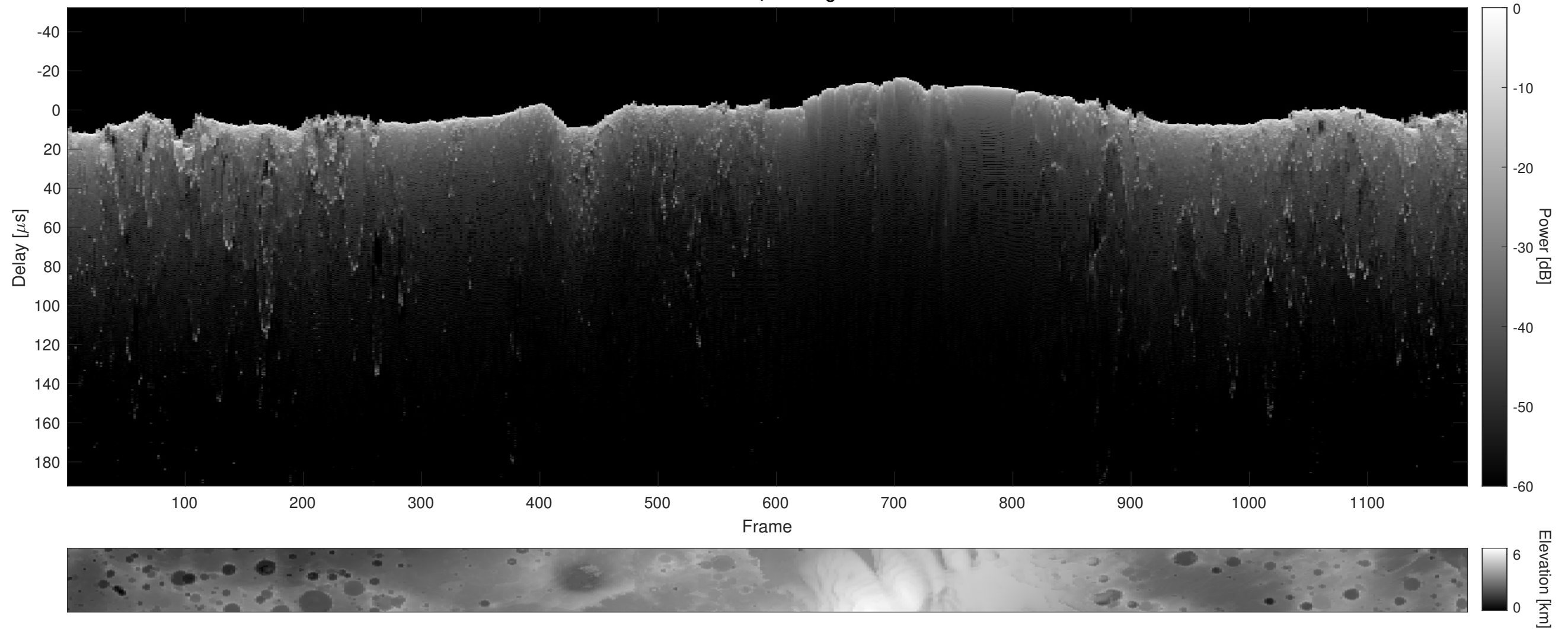
Orbit 10892, Cluttergram
