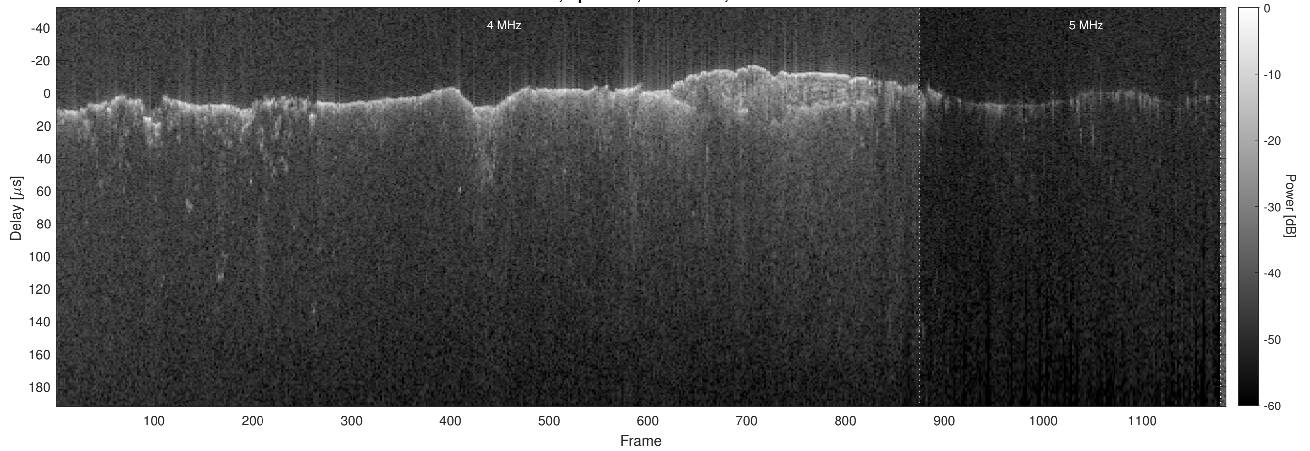
Orbit 10892, Optimized, No Window, Channel 2
