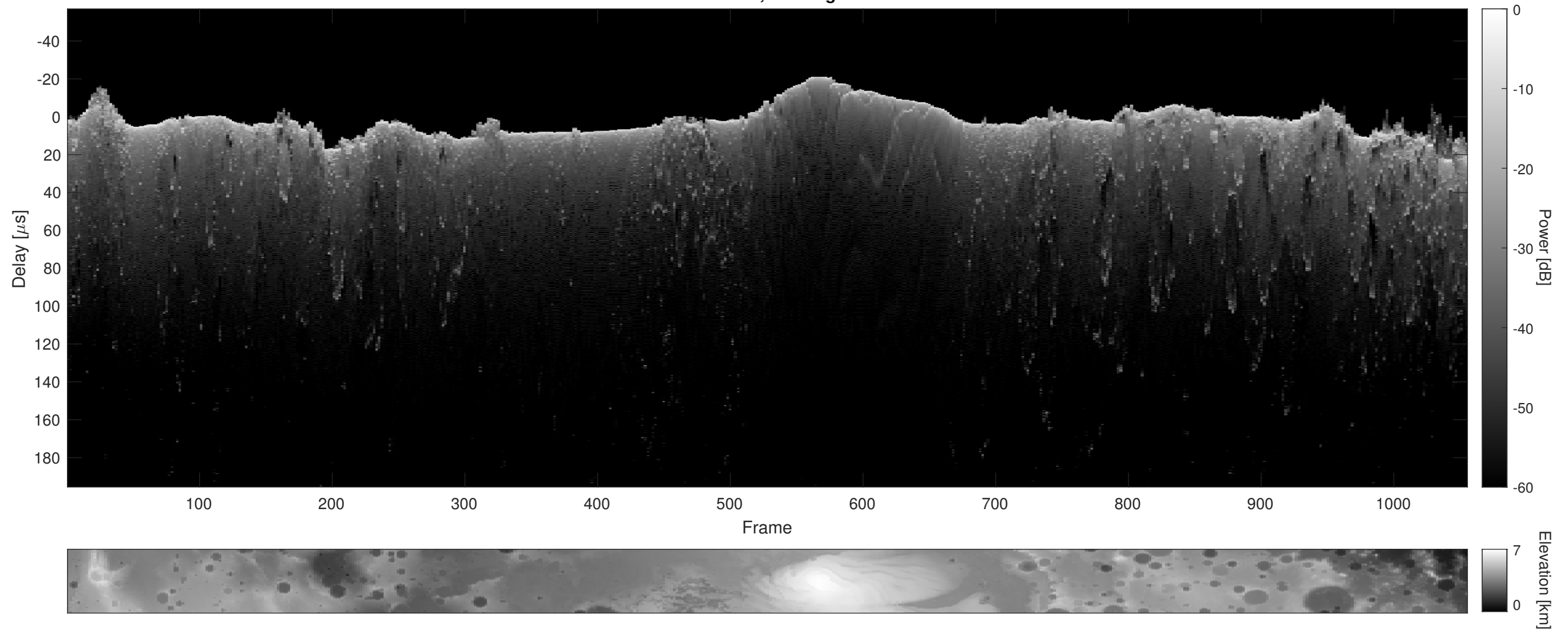
Orbit 10893, Cluttergram
