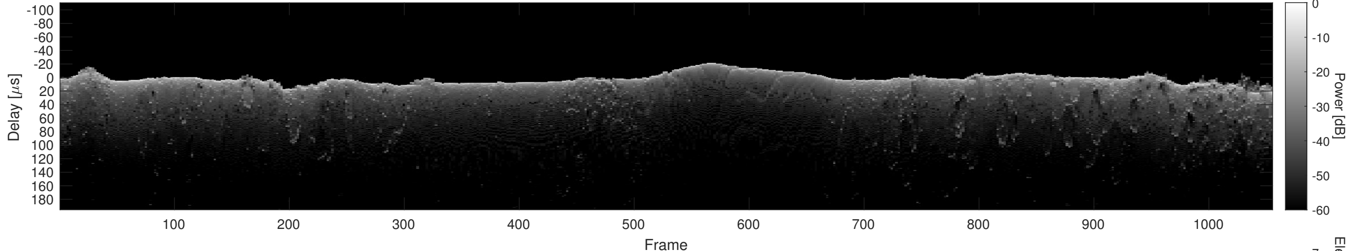
Orbit 10893, Cluttergram
