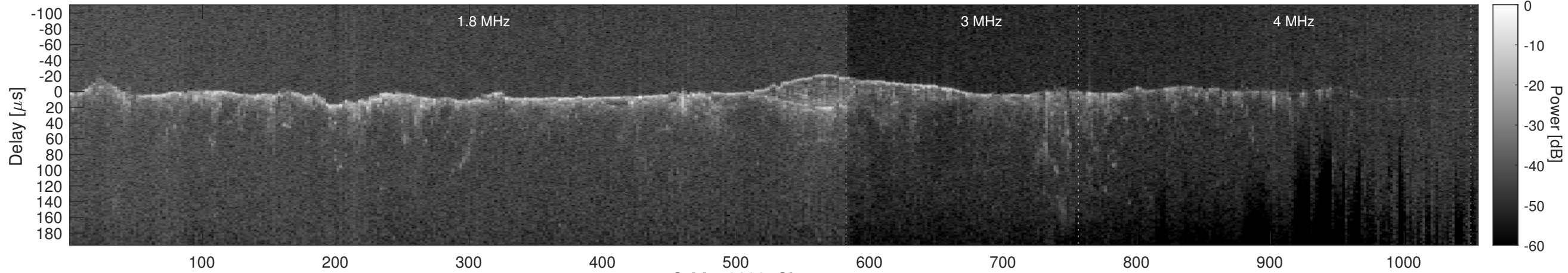
Orbit 10893, Cluttergram
