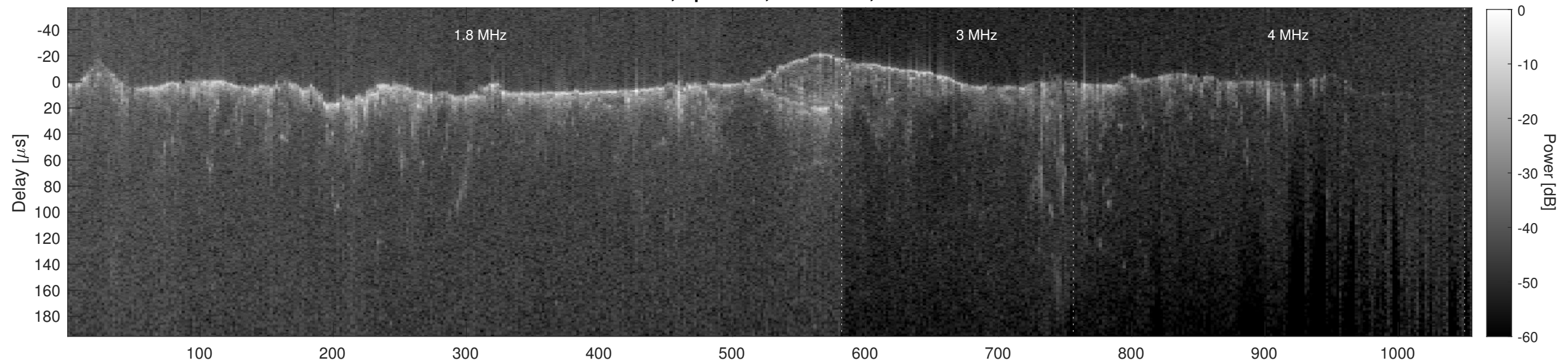
Orbit 10893, Cluttergram
