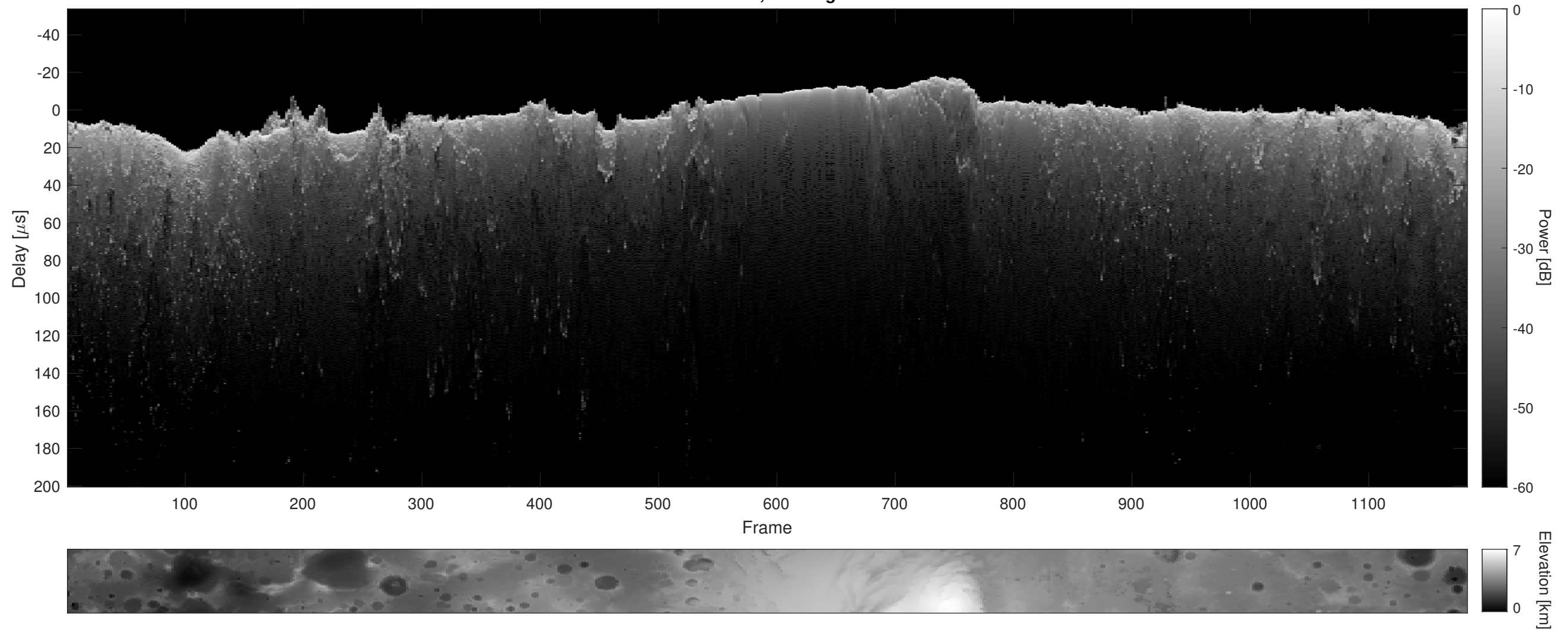
Orbit 10894, Cluttergram
