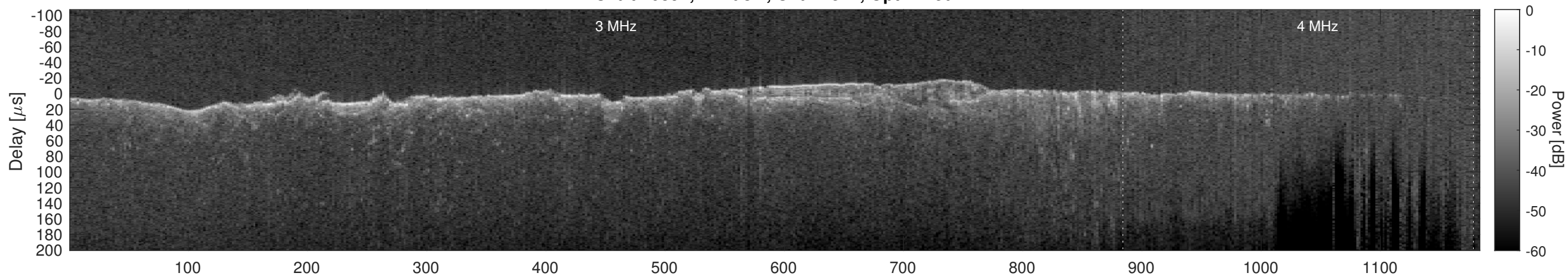
Orbit 10894, Cluttergram
