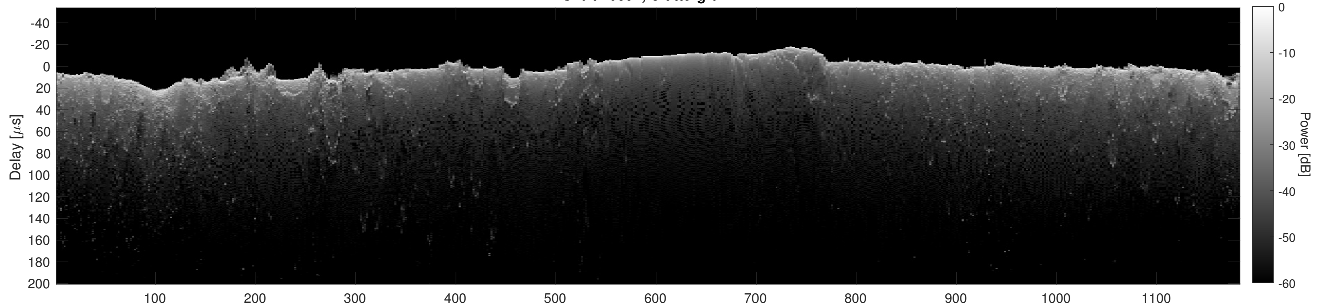
Orbit 10894, Cluttergram
