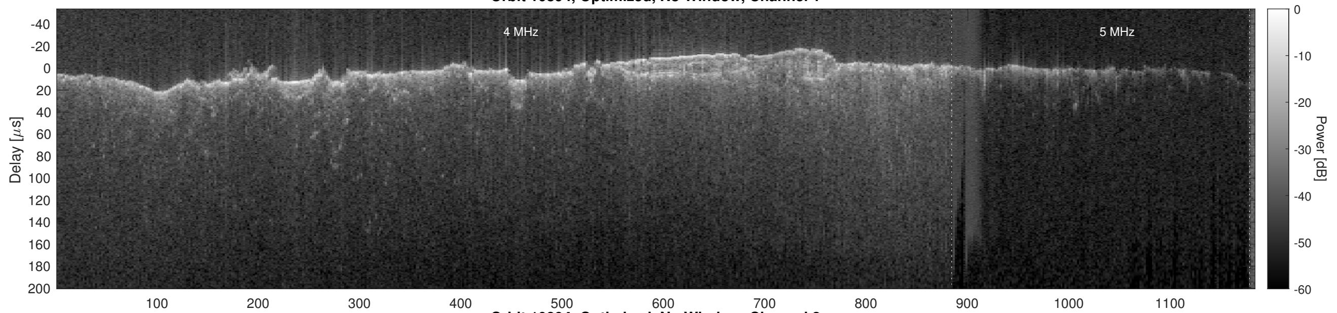
Orbit 10894, Optimized, No Window, Channel 2
