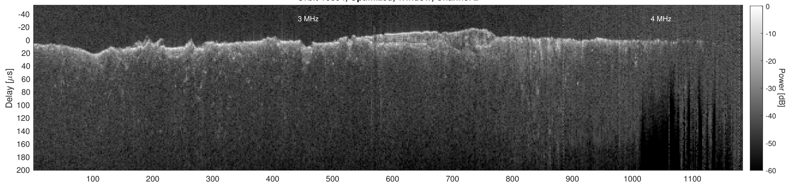
Orbit 10894, Cluttergram
