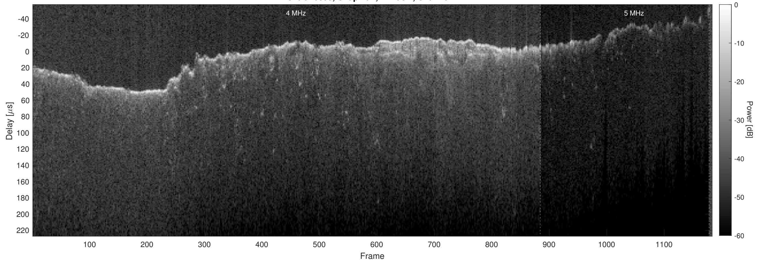
Orbit 10895, Chapman, Window, Channel 2
