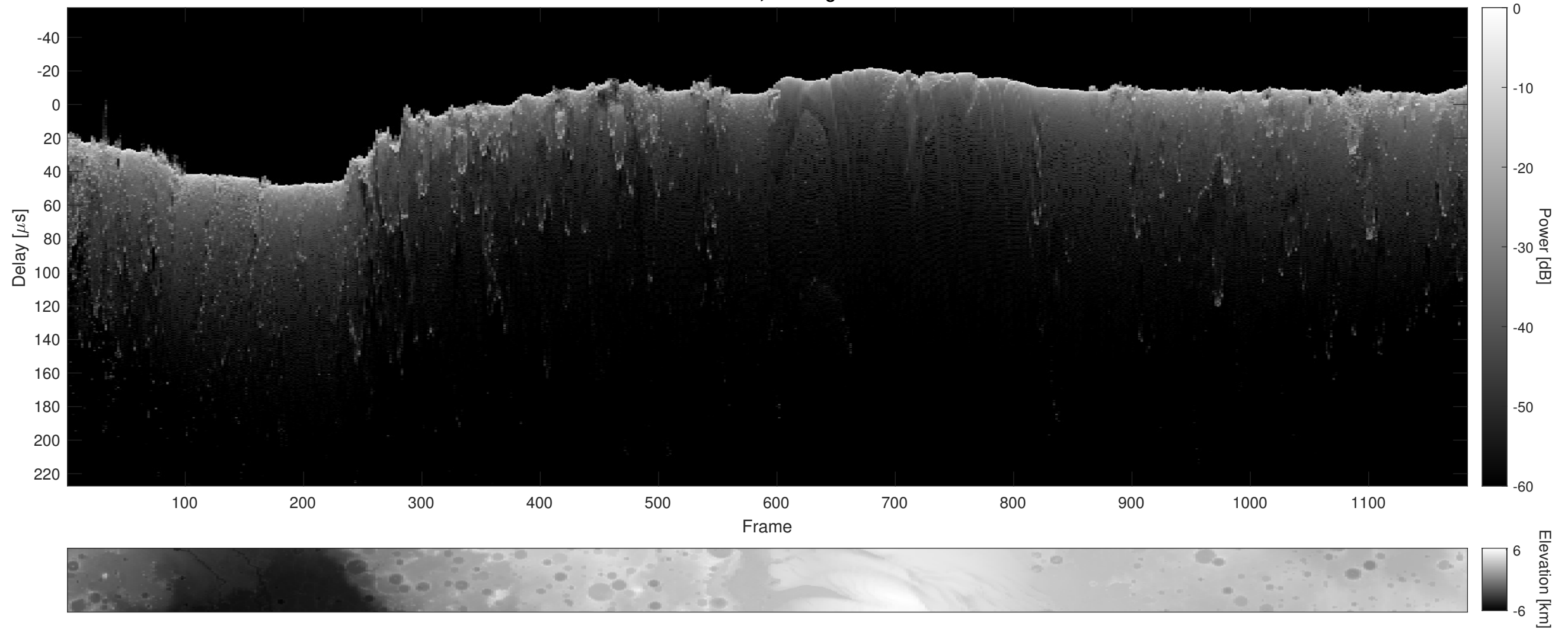
Orbit 10895, Cluttergram
