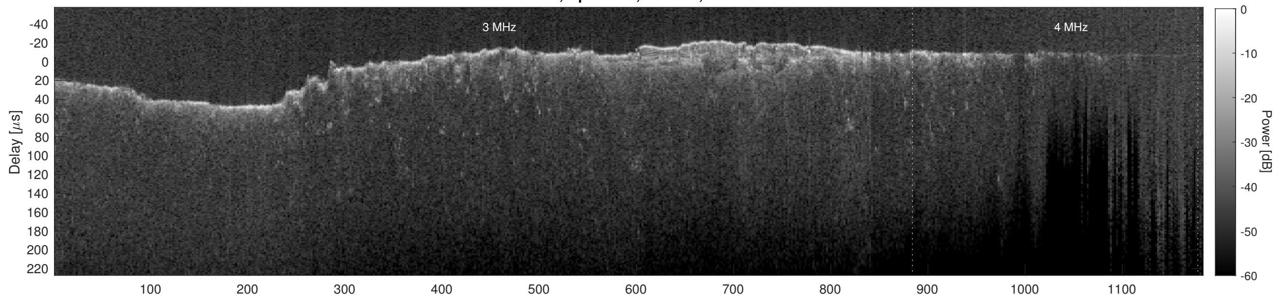
Orbit 10895, Cluttergram
