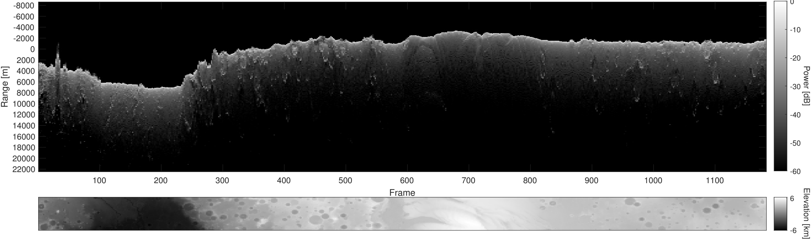
Orbit 10895, Depth-Corrected Cluttergram
