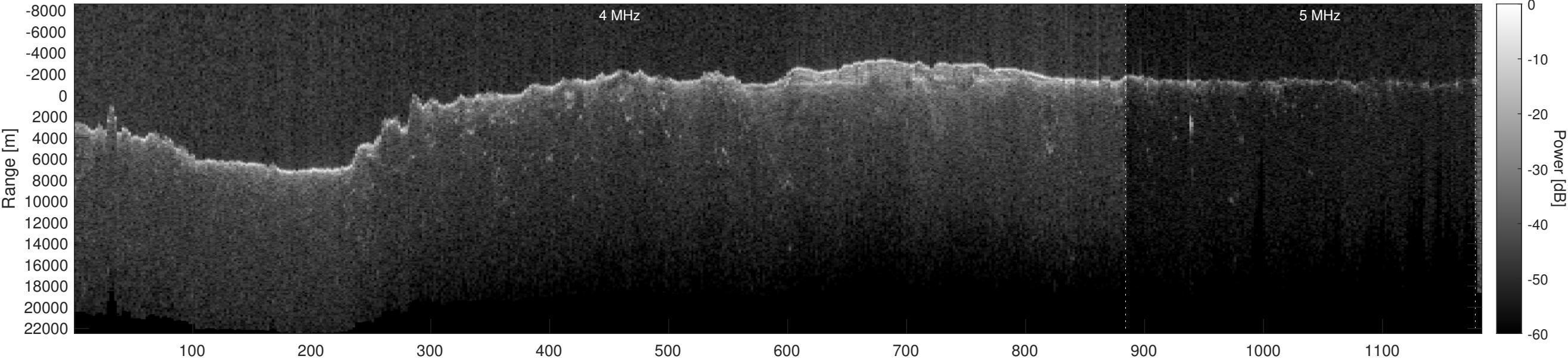
Orbit 10895, Optimized, Window, Depth-Corrected, Channel 2
