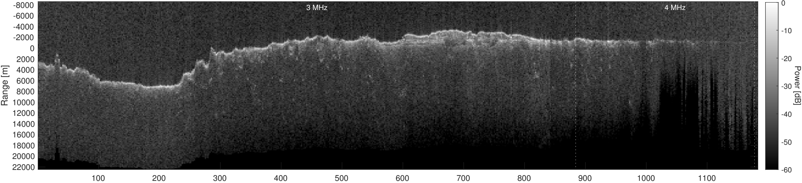
Orbit 10895, Depth-Corrected Cluttergram
