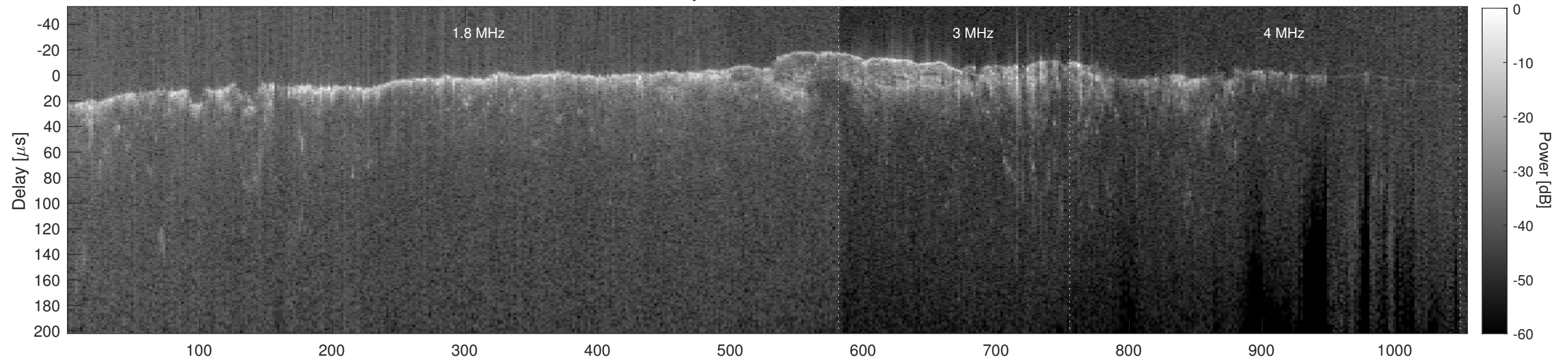
Orbit 10896, Cluttergram
