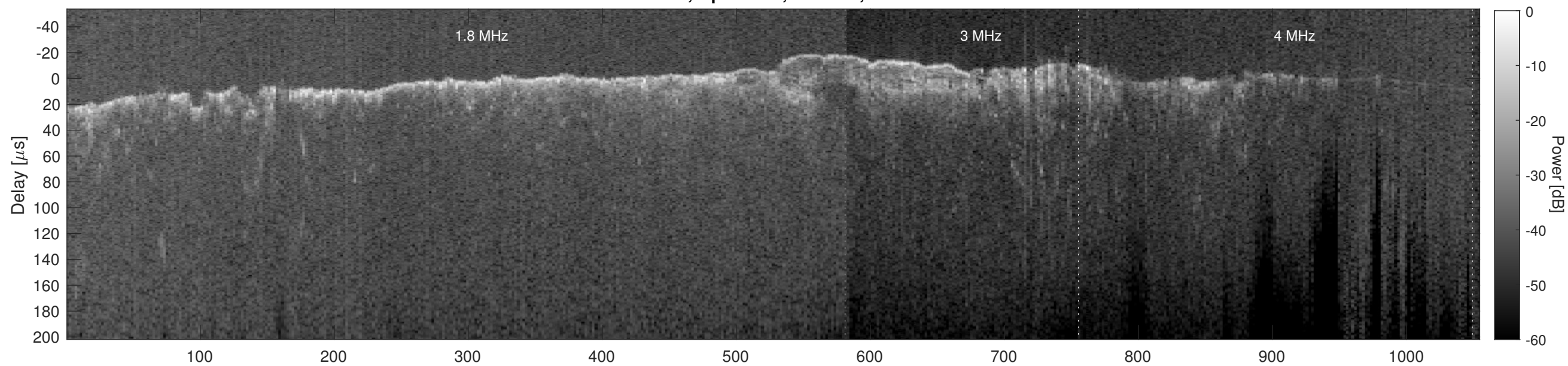
Orbit 10896, Cluttergram
