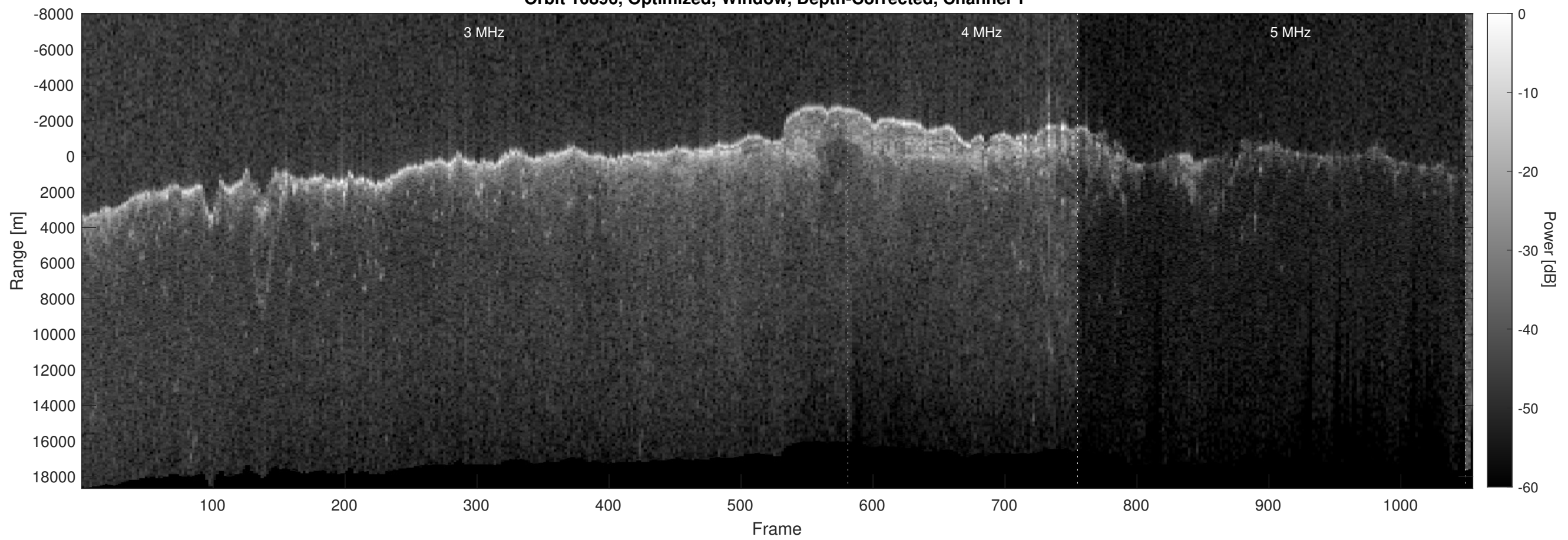
Orbit 10896, Optimized, Window, Depth-Corrected, Channel 2
