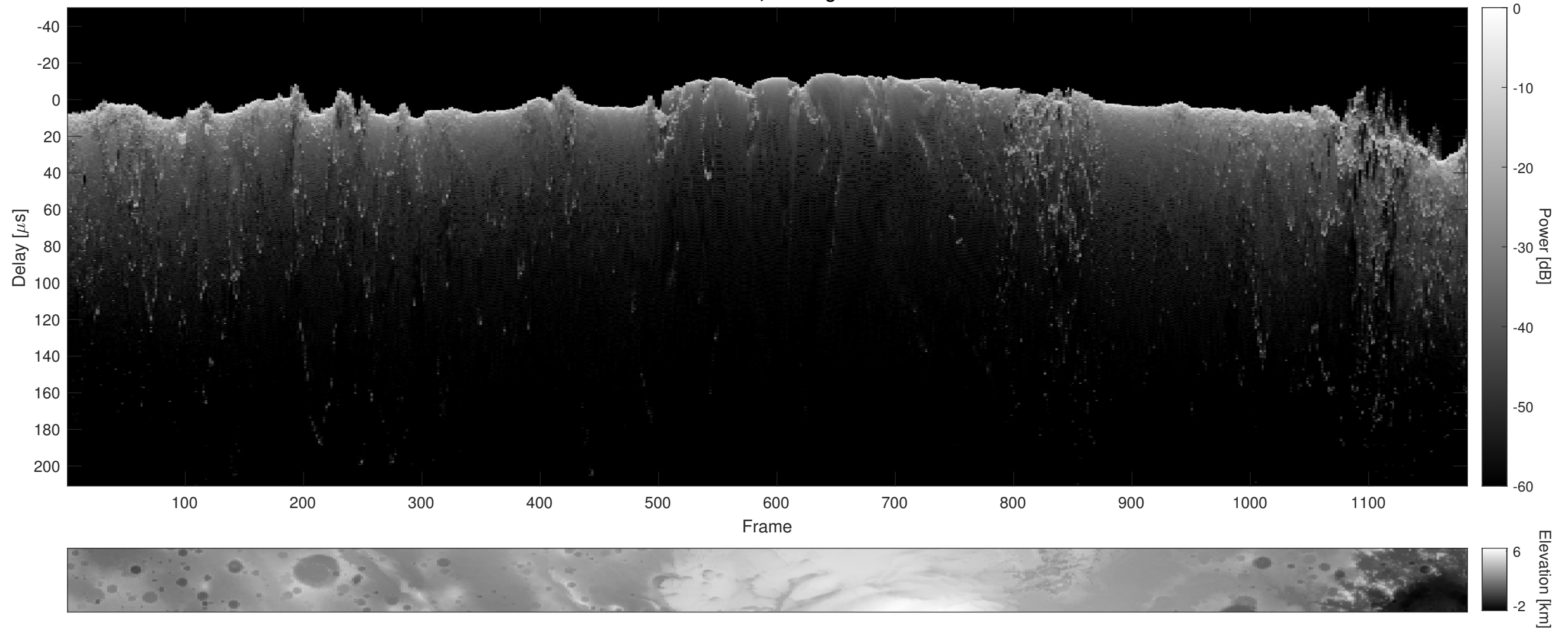
Orbit 10898, Cluttergram
