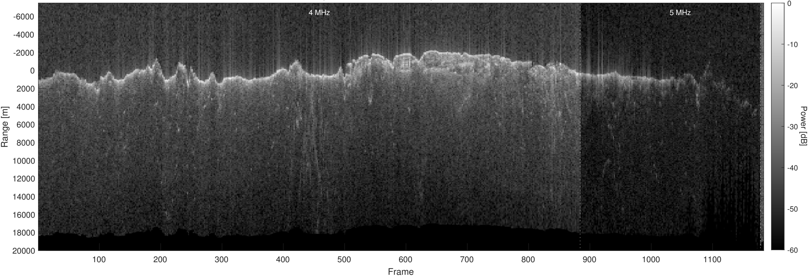
Orbit 10898, Optimized, No Window, Depth-Corrected, Channel 2
