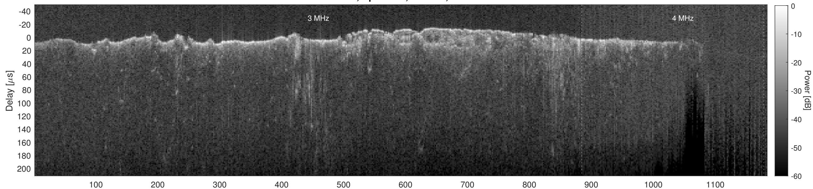
Orbit 10898, Cluttergram
