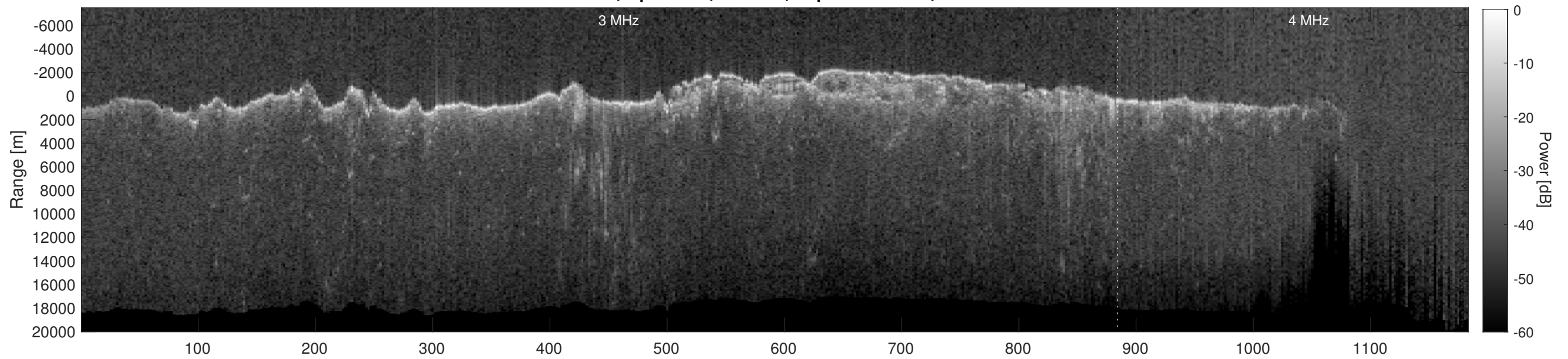
Orbit 10898, Depth-Corrected Cluttergram
