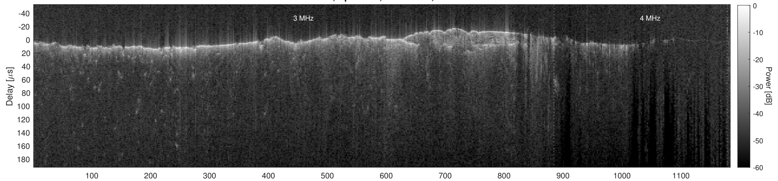
Orbit 10899, Cluttergram
