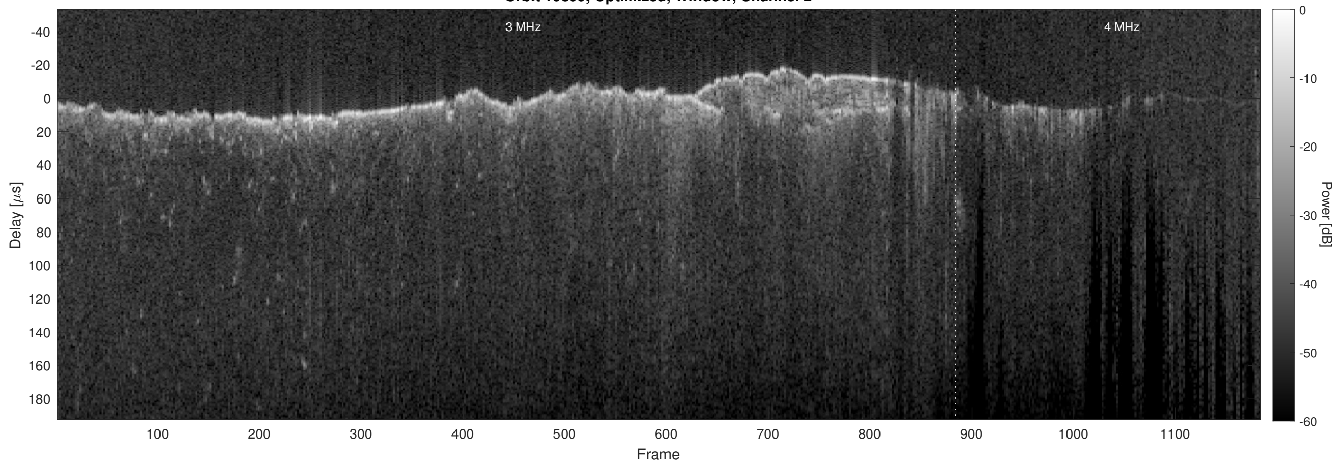
Orbit 10899, Optimized, Window, Channel 2
