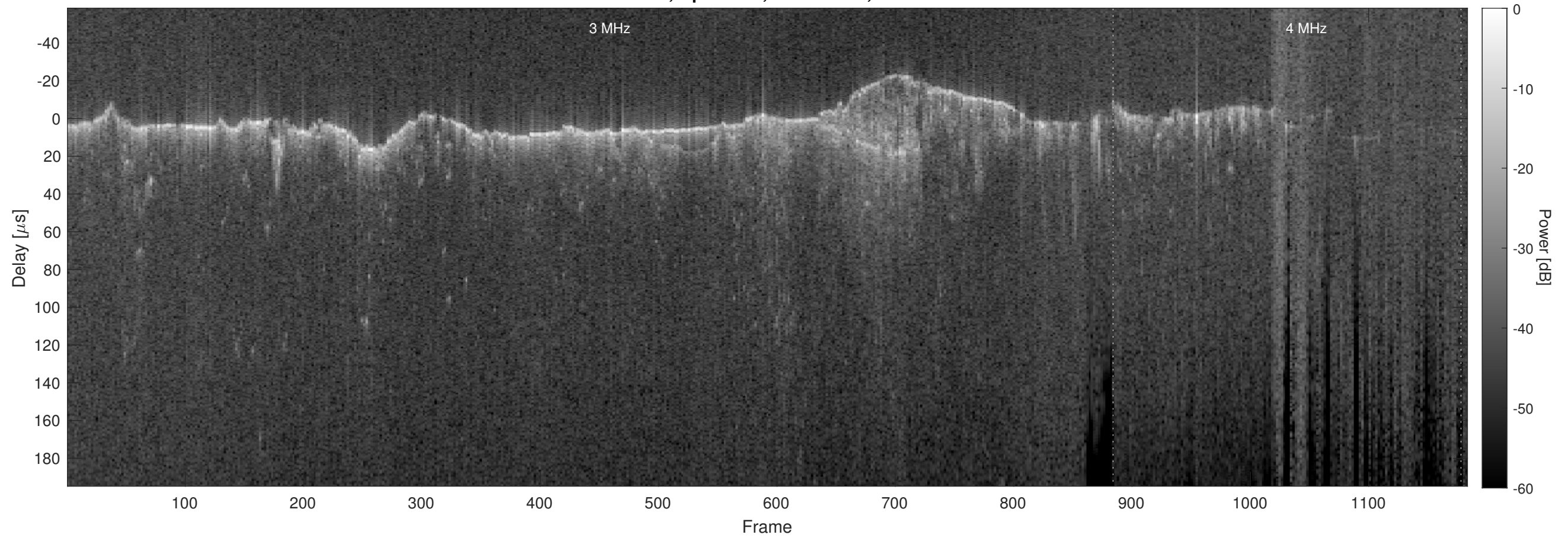
Orbit 10900, Optimized, No Window, Channel 2
