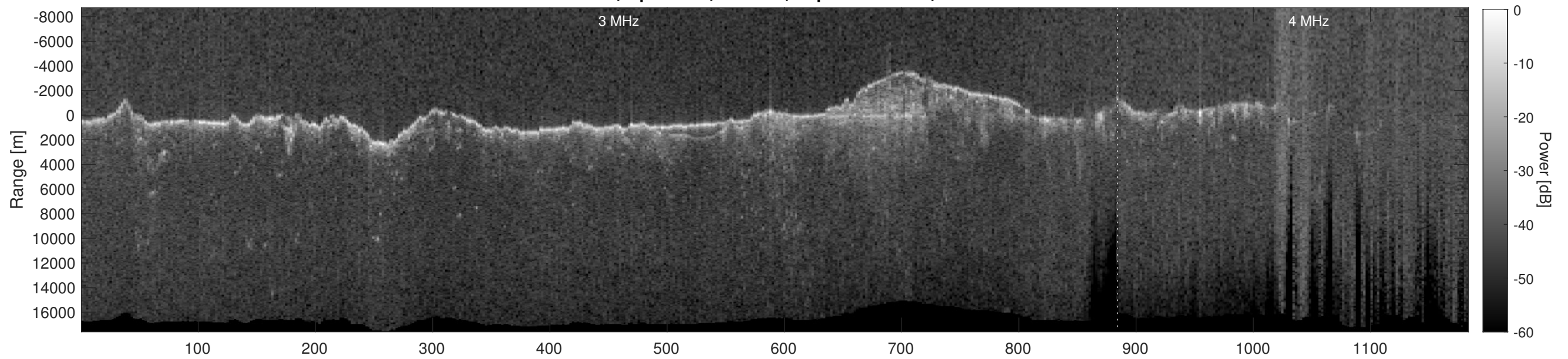
Orbit 10900, Depth-Corrected Cluttergram
