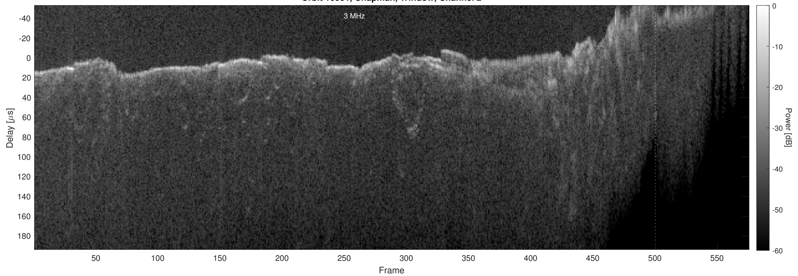
Orbit 10901, Chapman, Window, Channel 2
