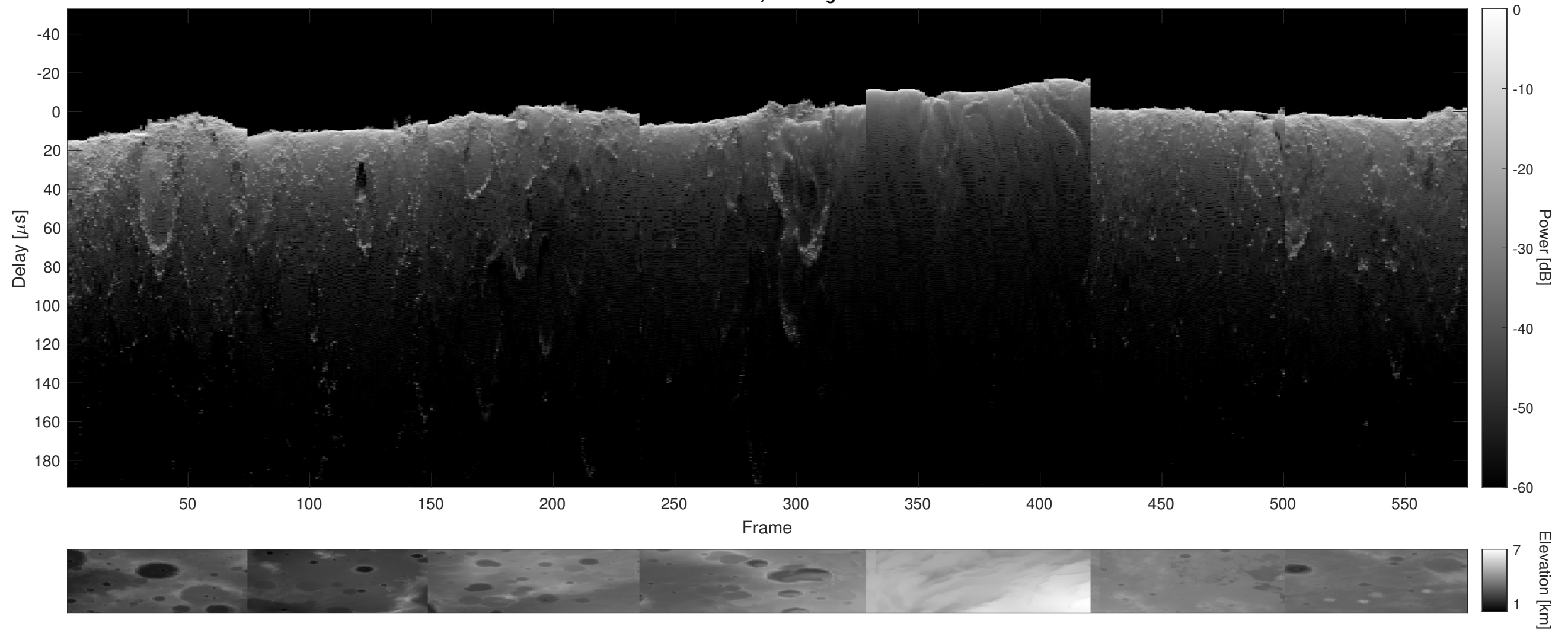
Orbit 10901, Cluttergram
