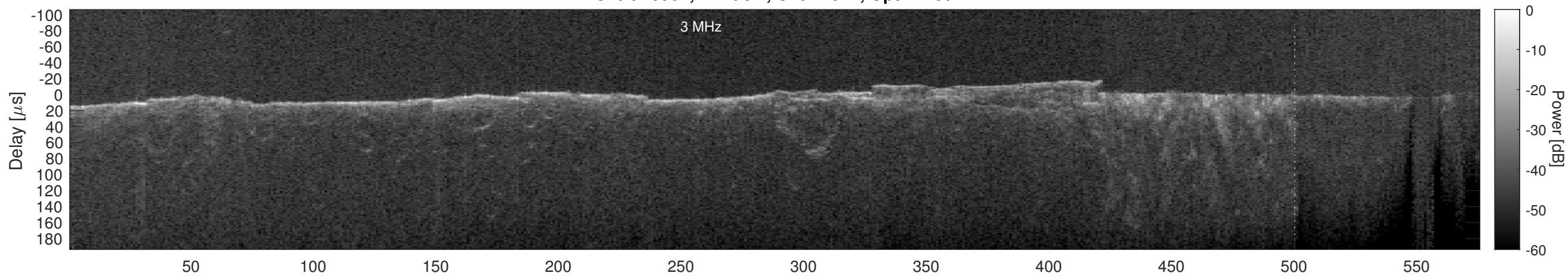
Orbit 10901, Cluttergram
