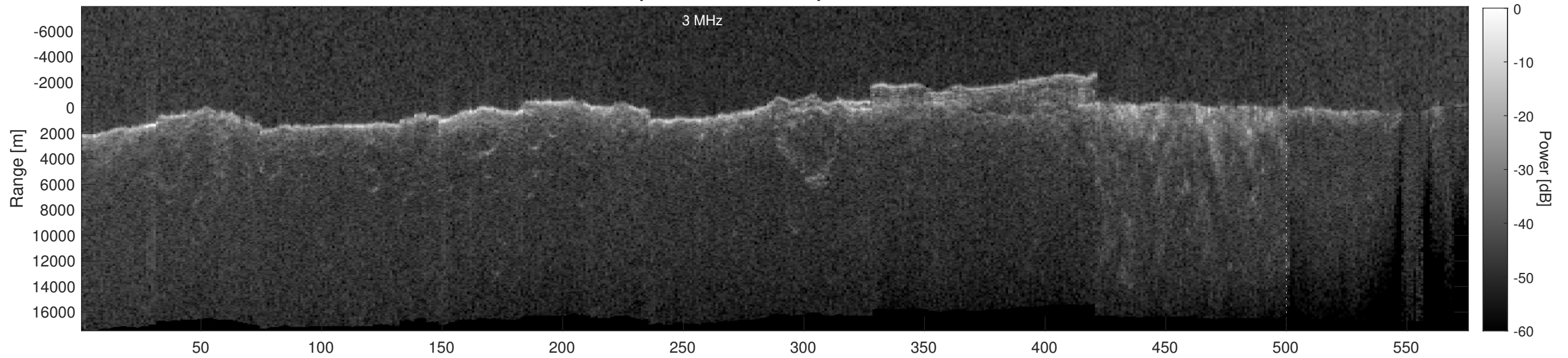
Orbit 10901, Depth-Corrected Cluttergram
