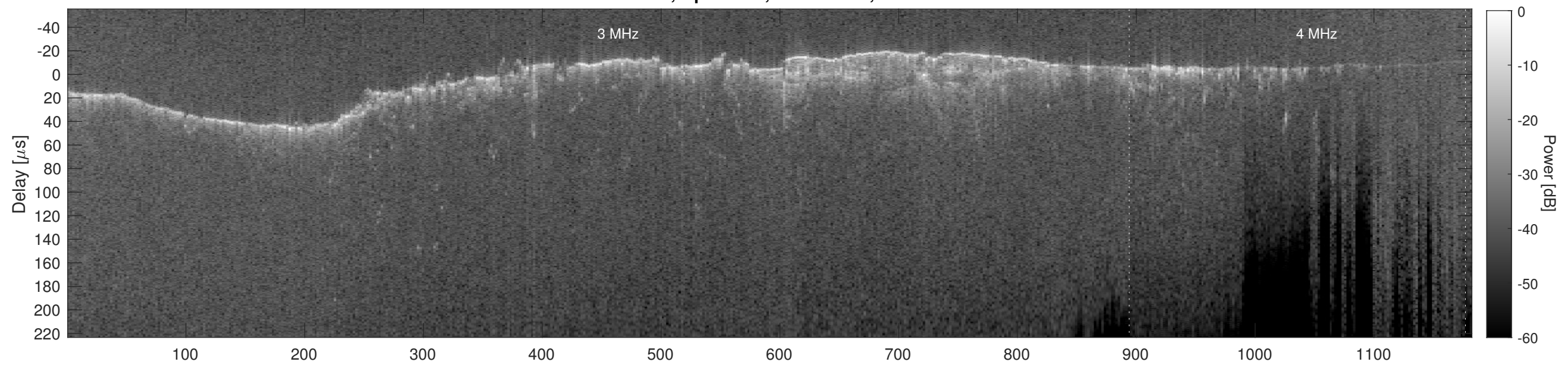
Orbit 10902, Cluttergram
