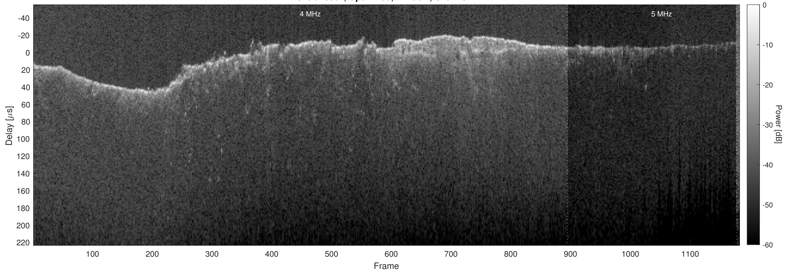
Orbit 10902, Optimized, Window, Channel 2
