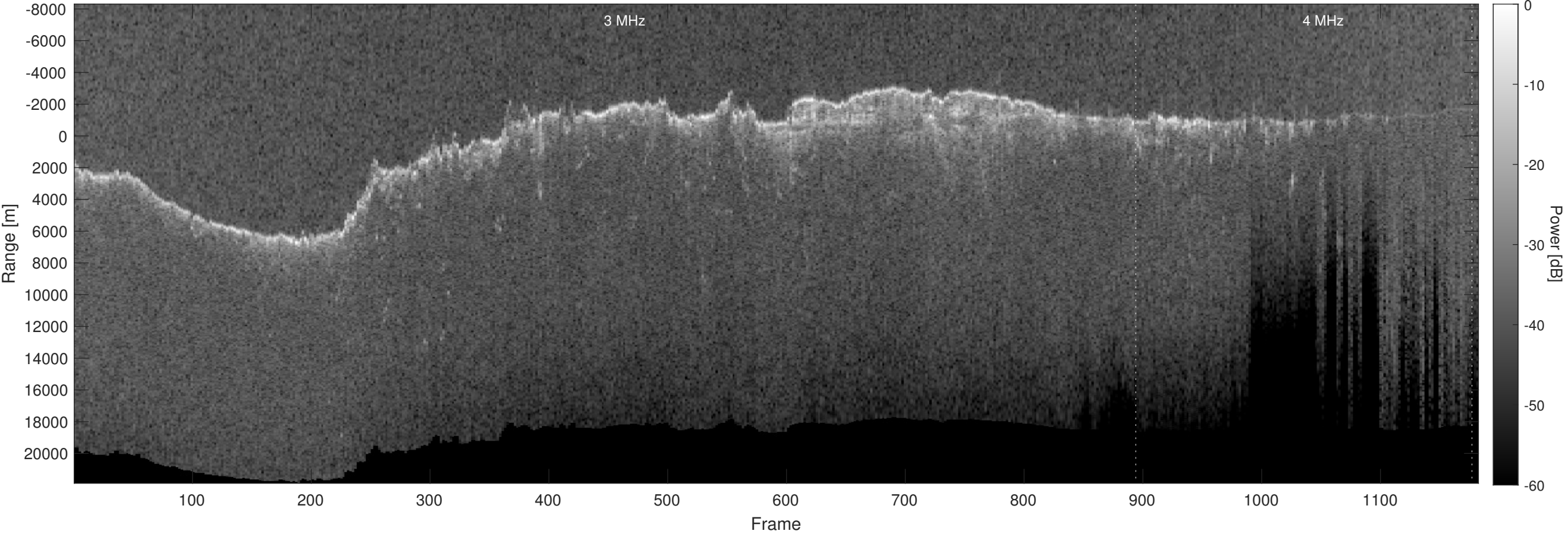
Orbit 10902, Optimized, Window, Depth-Corrected, Channel 2
