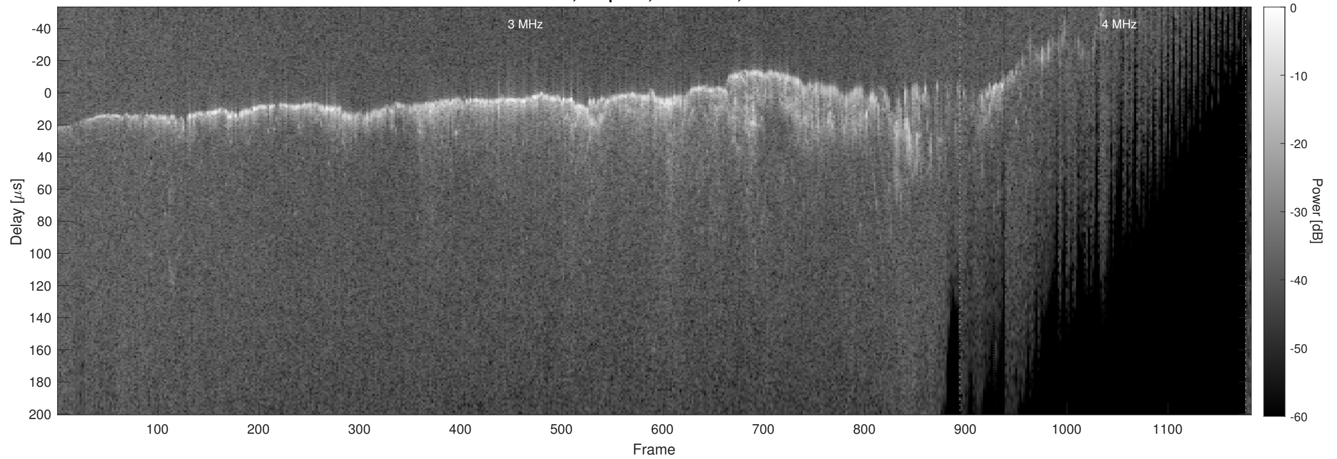
Orbit 10903, Chapman, No Window, Channel 2
