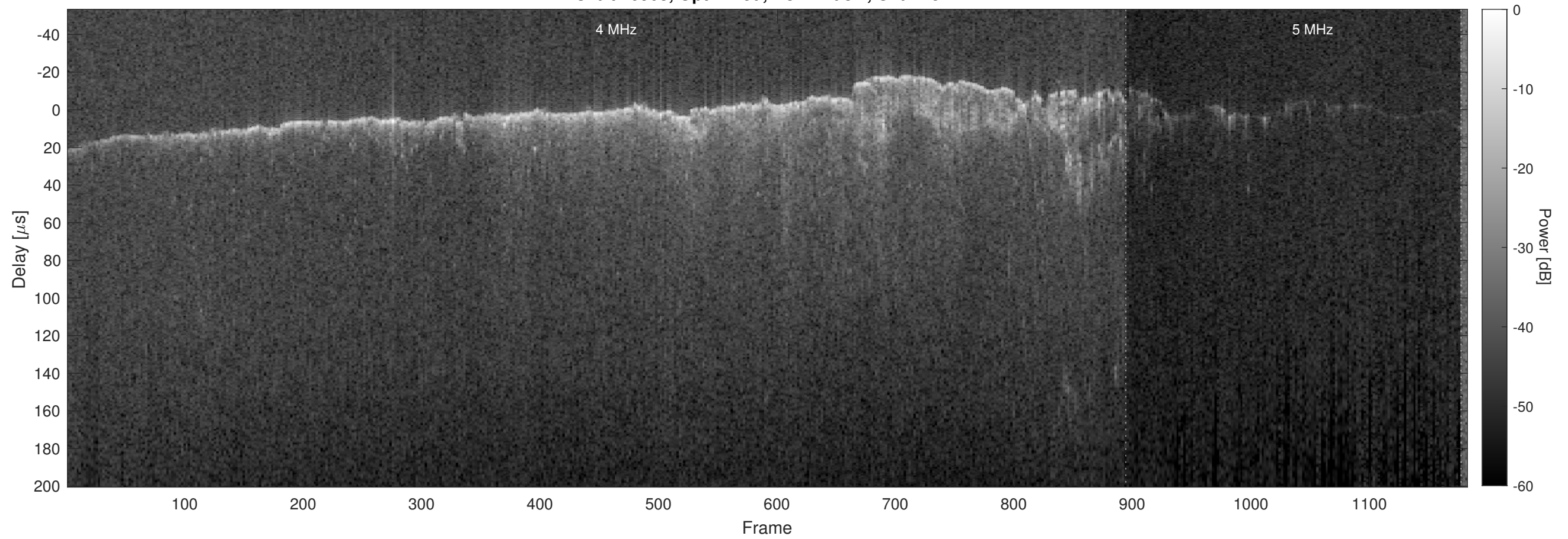
Orbit 10903, Optimized, No Window, Channel 2
