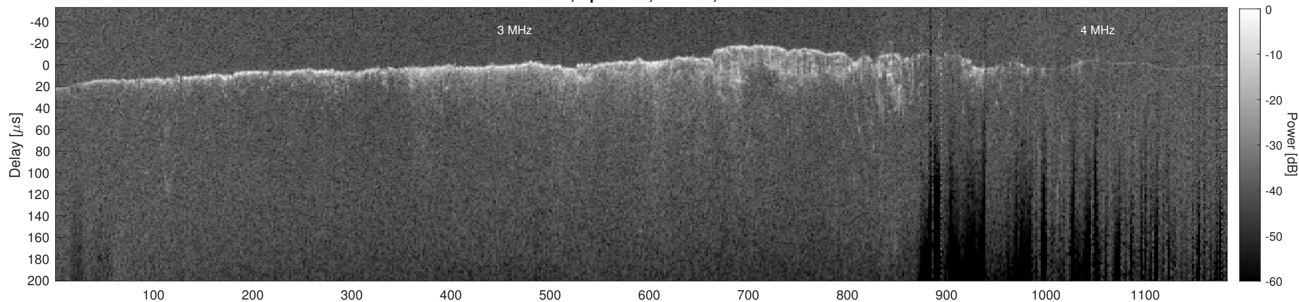
Orbit 10903, Cluttergram
