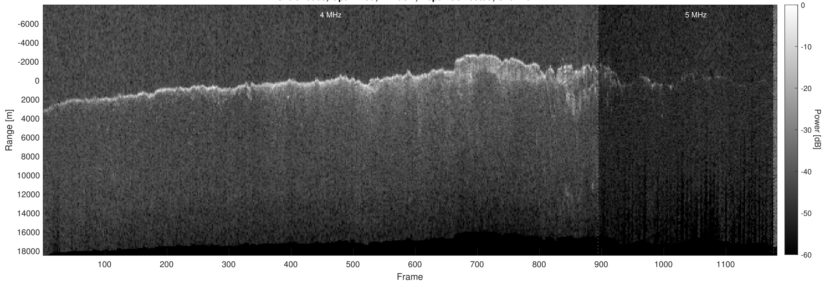
Orbit 10903, Optimized, Window, Depth-Corrected, Channel 2
