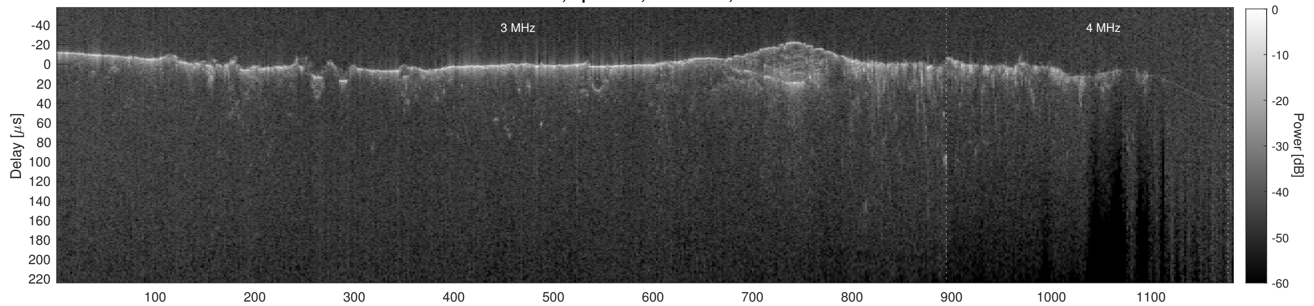
Orbit 10904, Cluttergram
