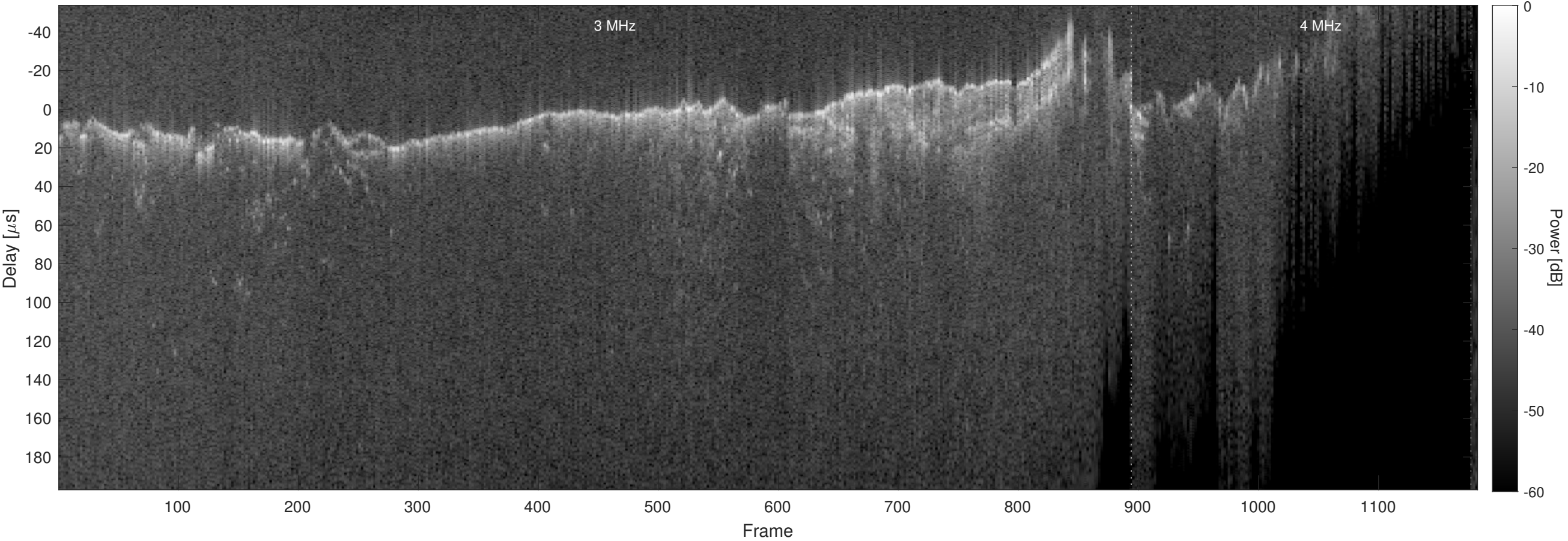
Orbit 10906, Chapman, No Window, Channel 2
