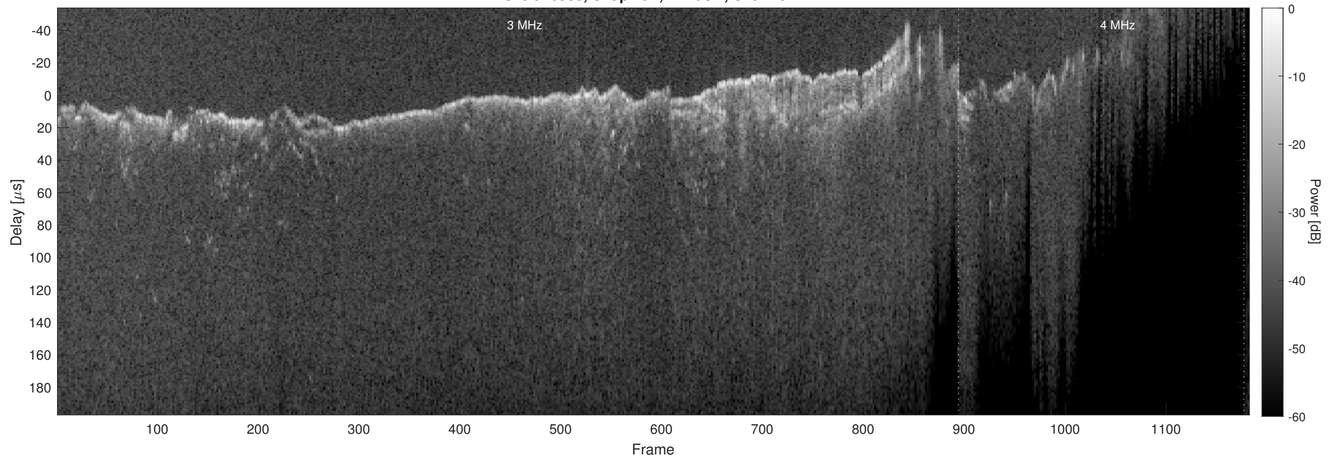
Orbit 10906, Chapman, Window, Channel 2
