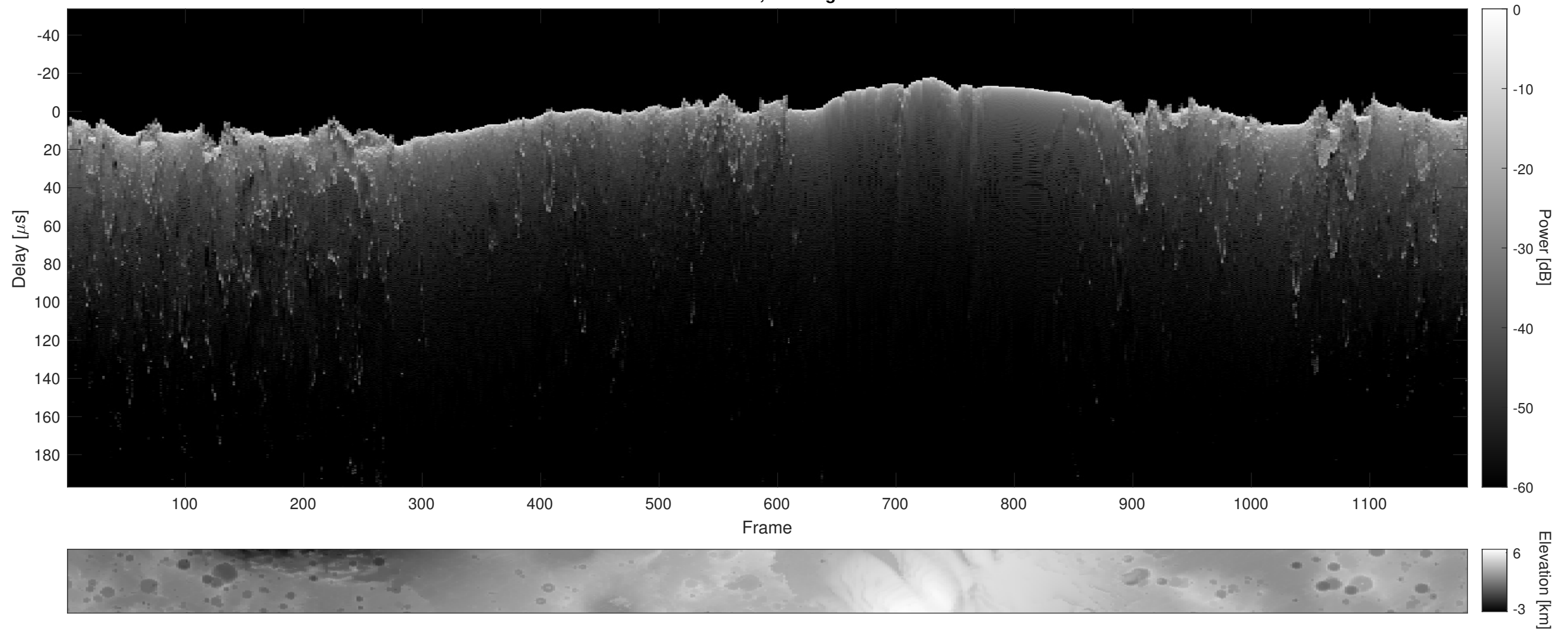
Orbit 10906, Cluttergram
