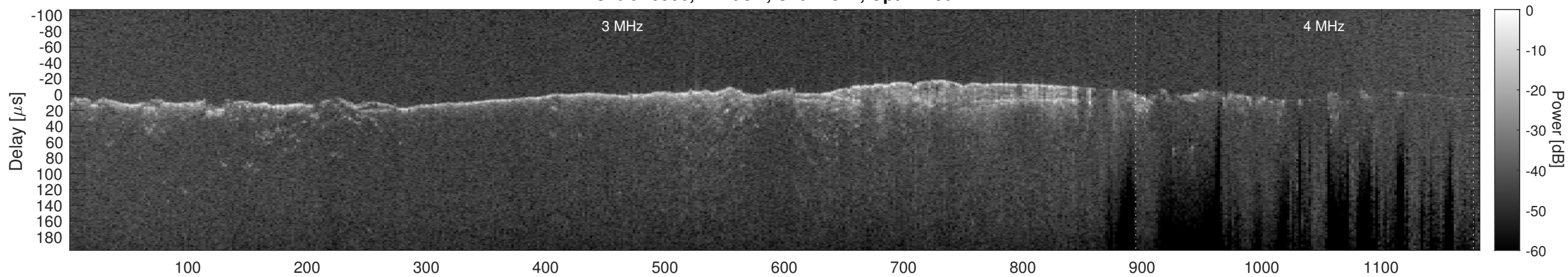
Orbit 10906, Cluttergram
