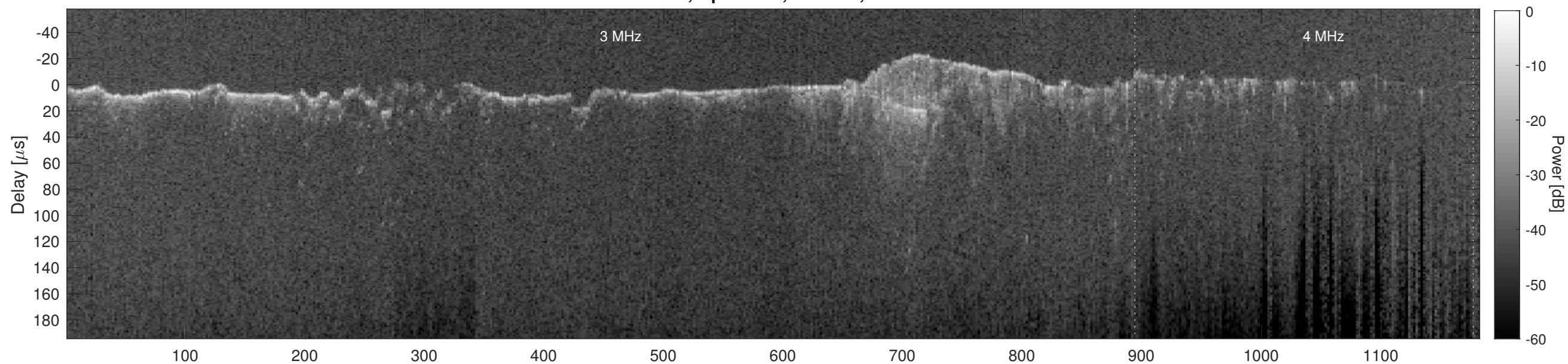
Orbit 10907, Cluttergram
