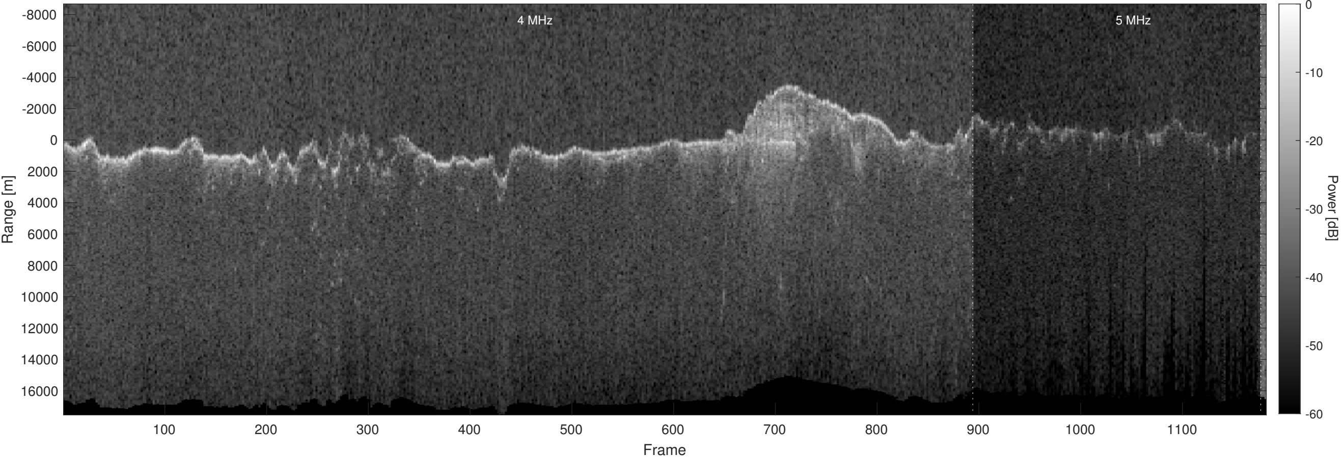
Orbit 10907, Optimized, Window, Depth-Corrected, Channel 2
