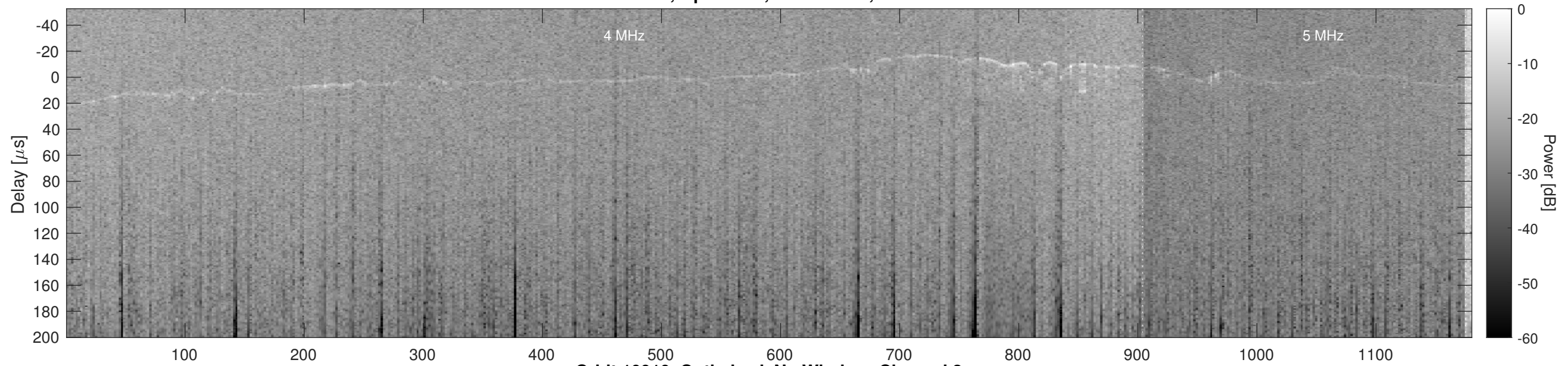
Orbit 10910, Optimized, No Window, Channel 2
