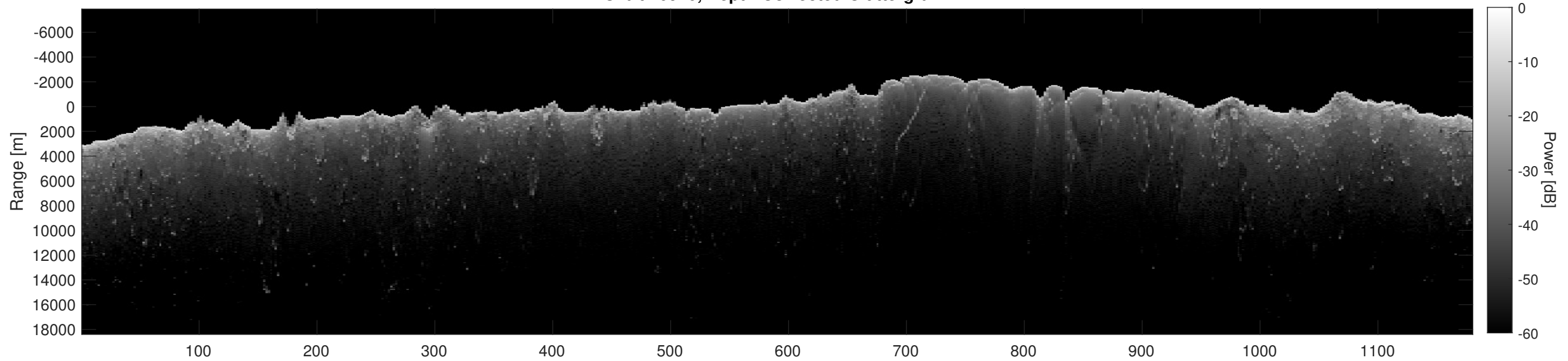
Orbit 10910, Depth-Corrected Cluttergram
