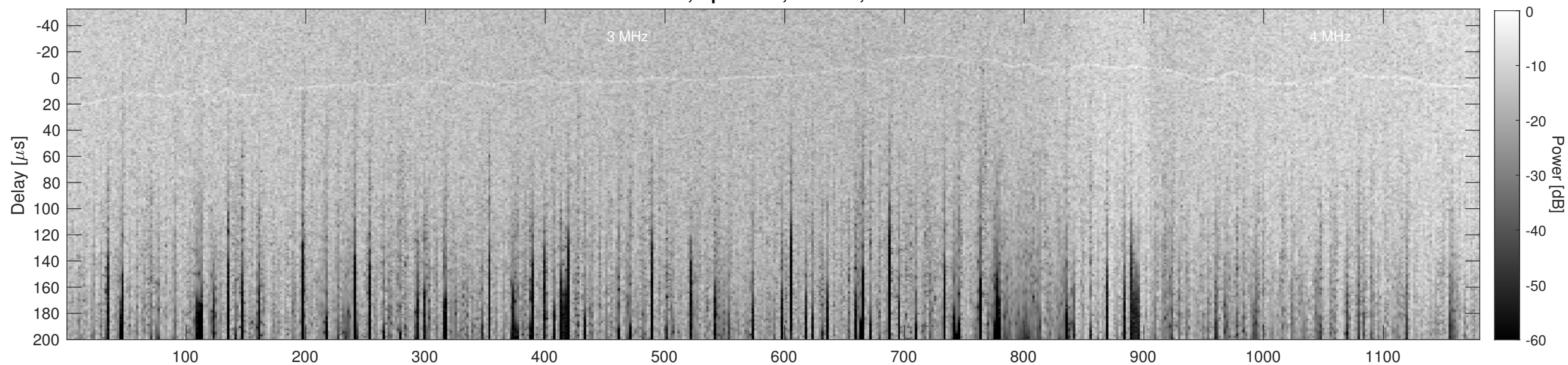
Orbit 10910, Cluttergram
