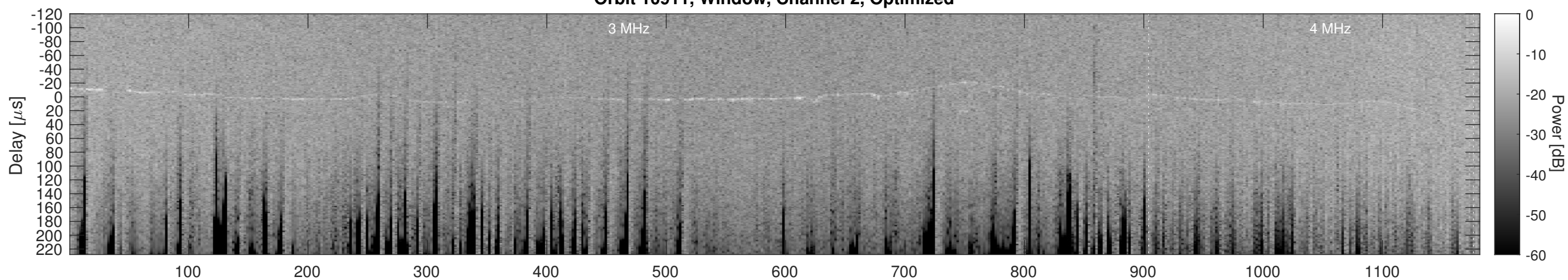
Orbit 10911, Cluttergram
