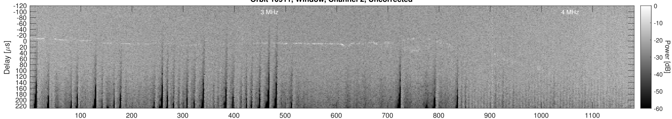
Orbit 10911, Window, Channel 2, Chapman
