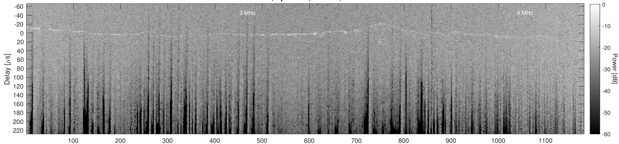
Orbit 10911, Cluttergram
