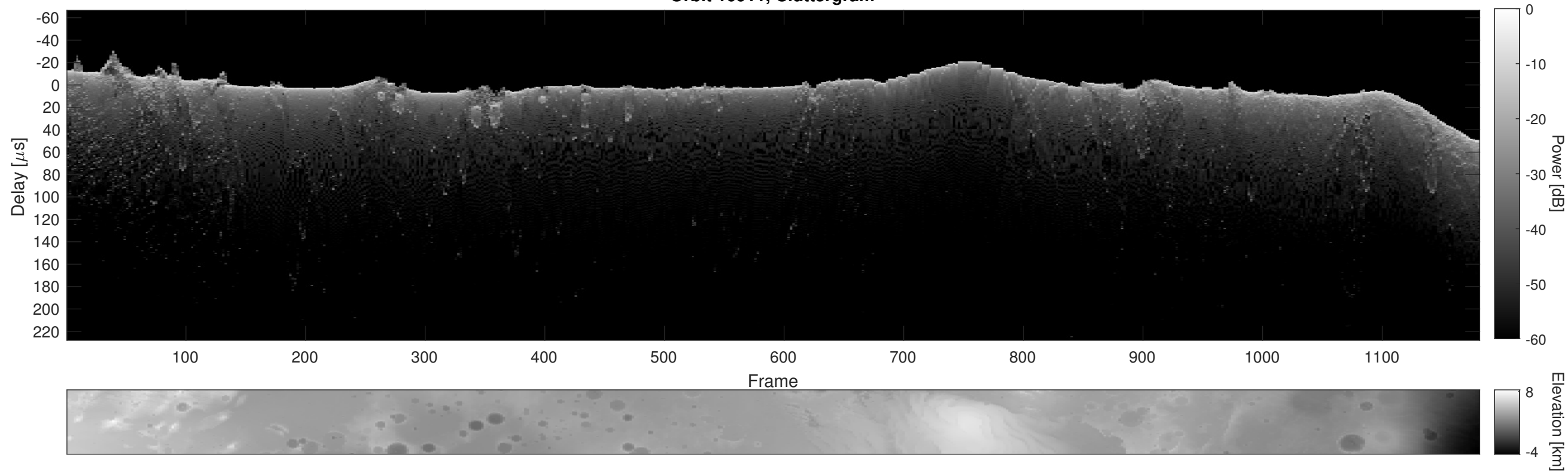
Orbit 10911, Cluttergram
