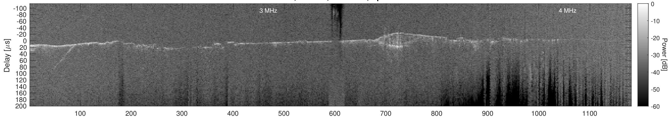
Orbit 10914, Cluttergram
