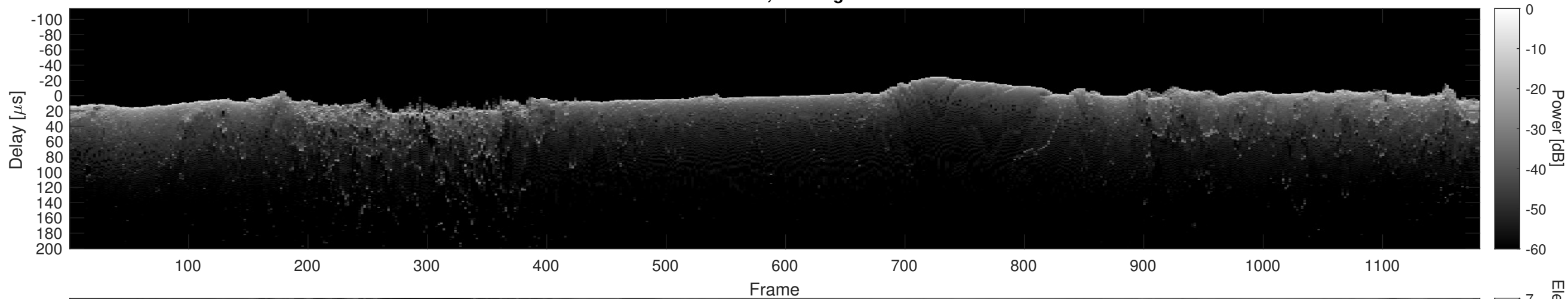
Orbit 10914, Cluttergram
