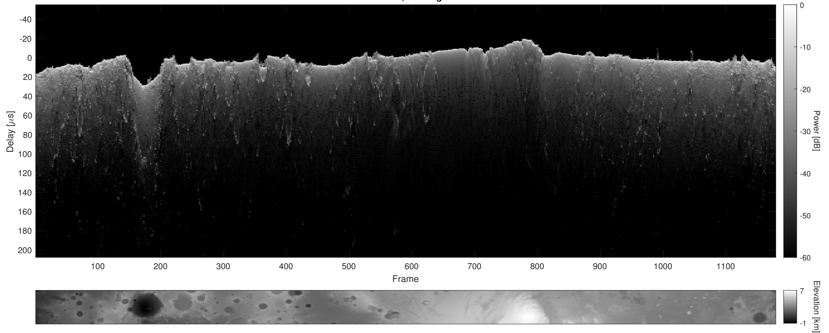
Orbit 10915, Cluttergram
