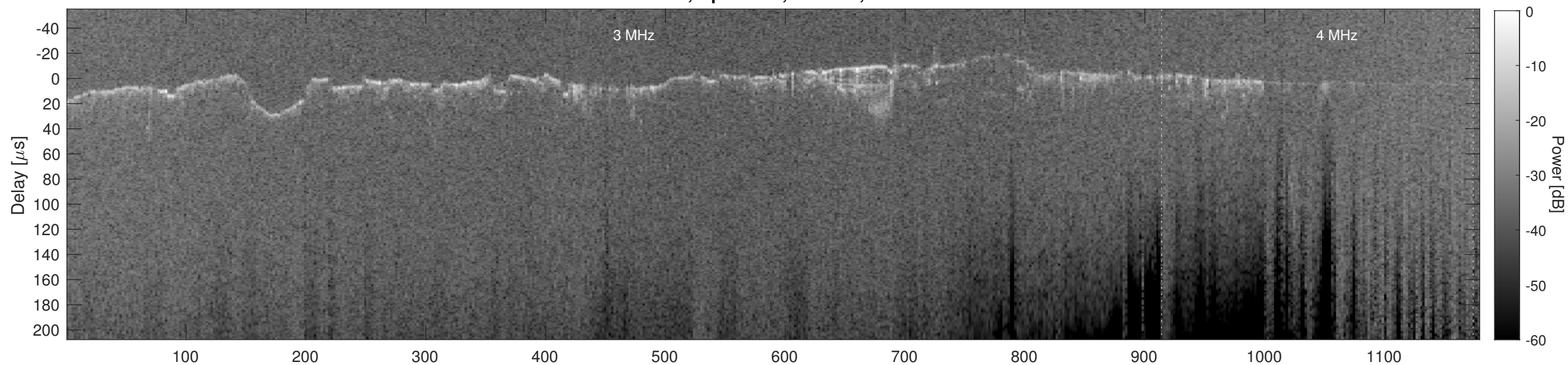
Orbit 10915, Cluttergram
