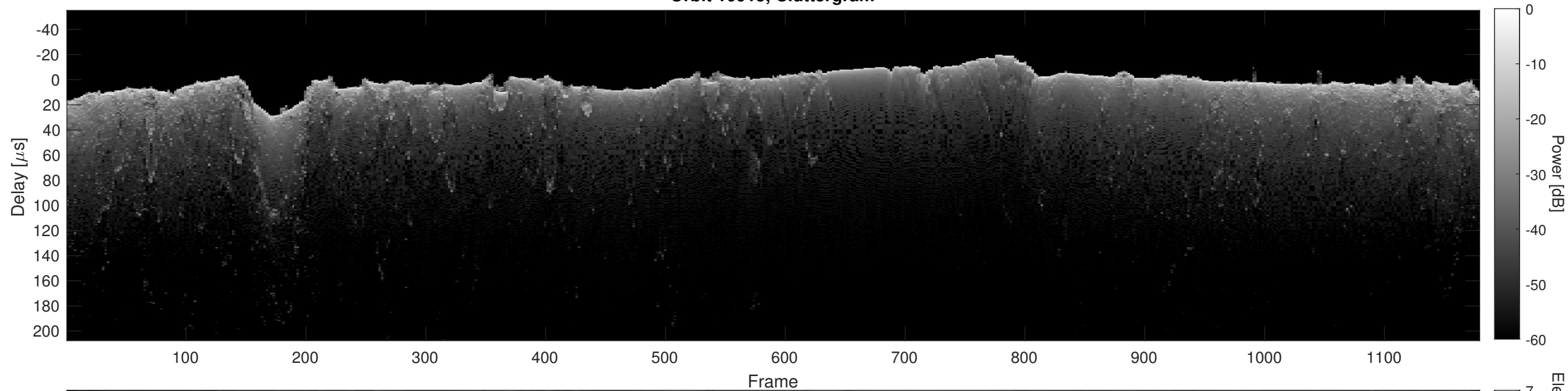
Orbit 10915, Cluttergram
